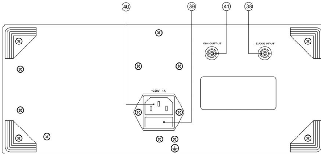
Fig. 5-2 Painel traseiro
